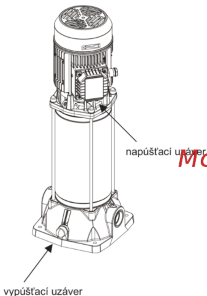
Obr. 5 KVC - KVCX
