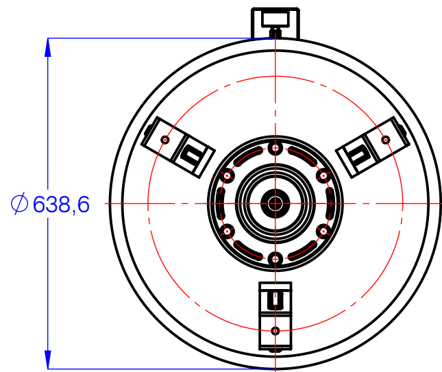
VIEW B
